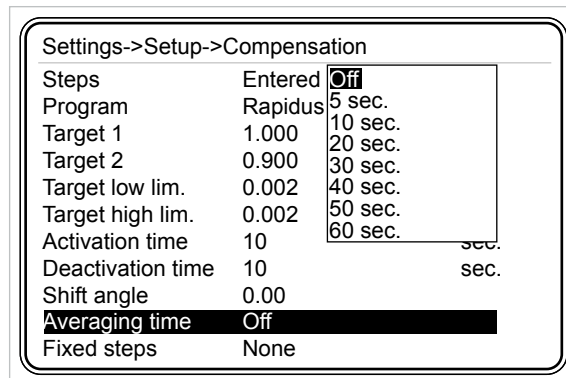
Fig. 3-35 Averaging Time Menu
