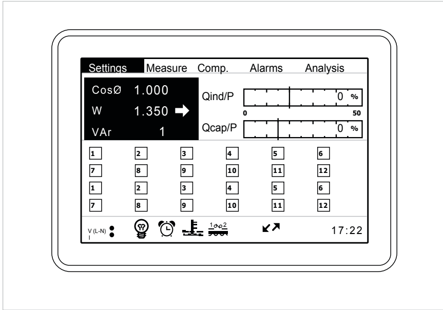
Fig. 1-3 Selected Step for RAPIDUS 212R
