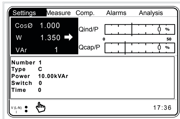
Fig. 3-33 Manual mod for RAPIDUS 212R
