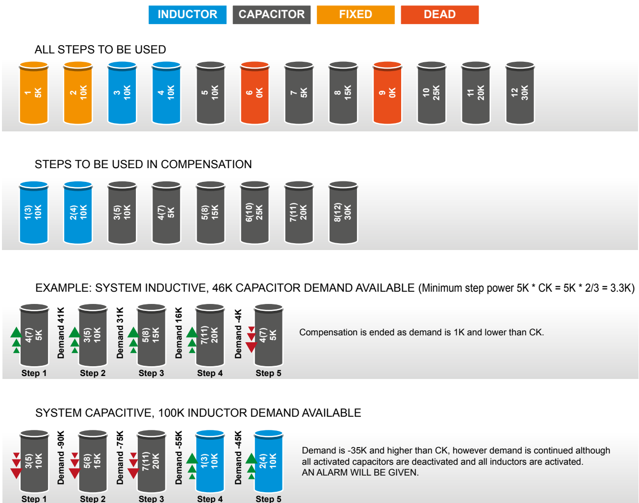
Fig. 3-28 RAPIDUS Asc. Sequential Mode
