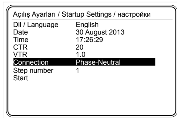
Fig. 3-8 Connection
