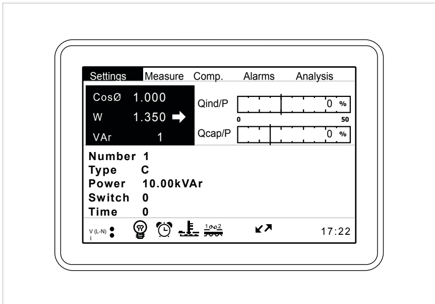
Fig. 1-4 Step Information Screen for RAPIDUS 212R
