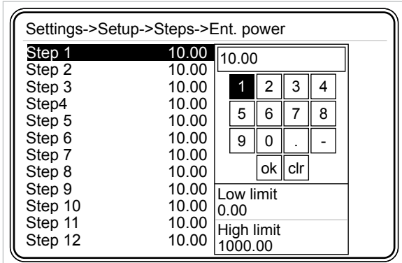
Fig. 3-21 Ent. Power Menu
