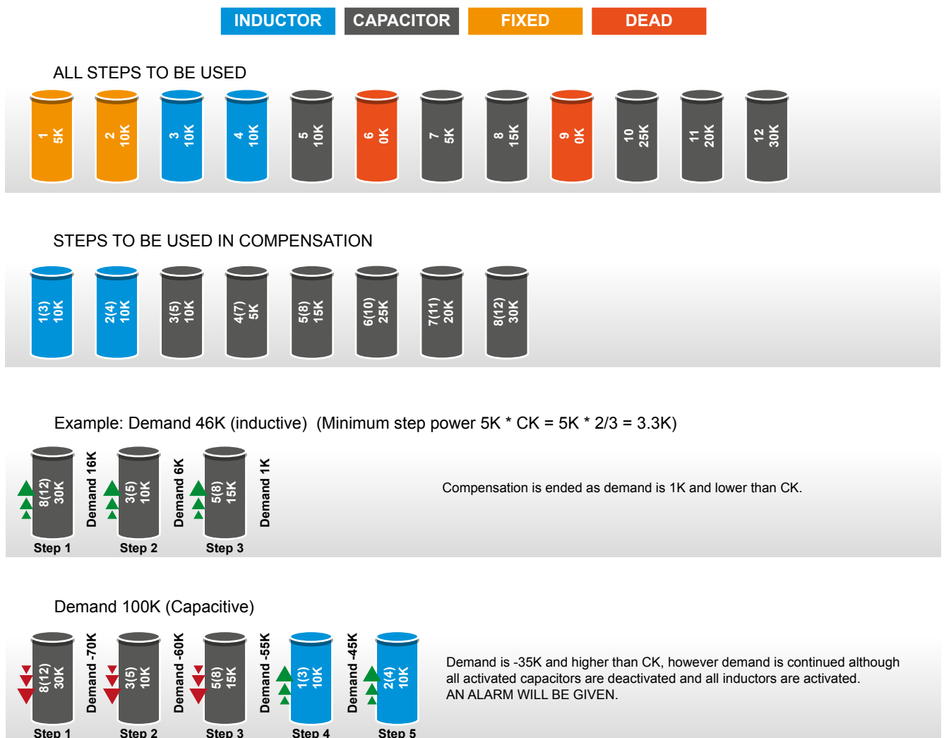
Fig. 3-29 RAPIDUS Des. Sequential Mode
