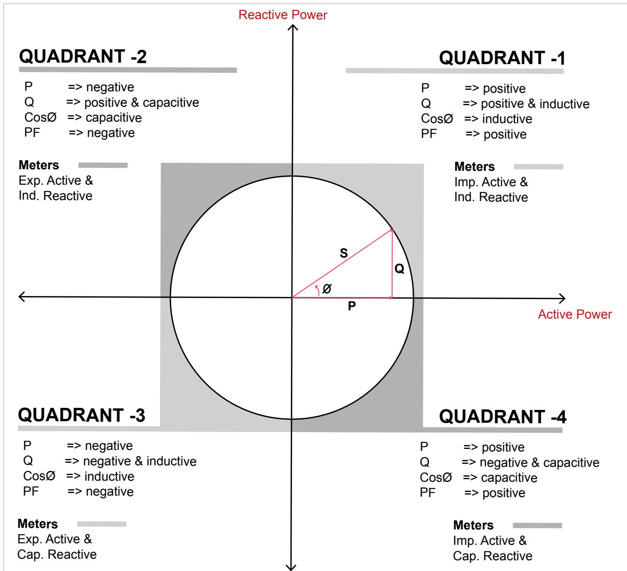
Fig. 1-5 Four-Quadrant Representation
