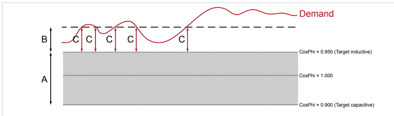
Fig. 3-27 RAPIDUS Mode Compensation Steps
