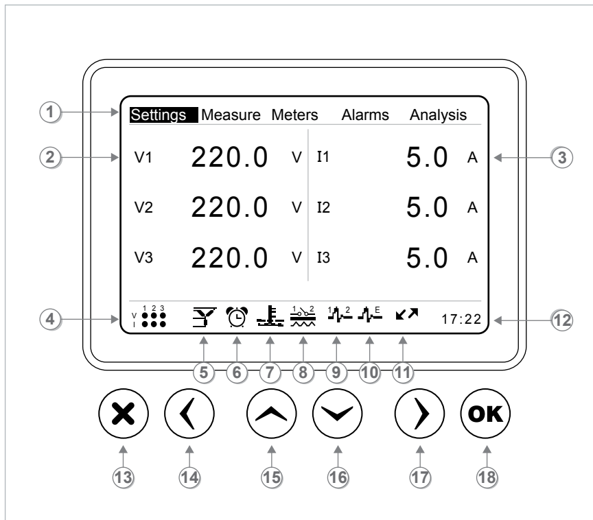
Figure 1-1 KLEA Display
