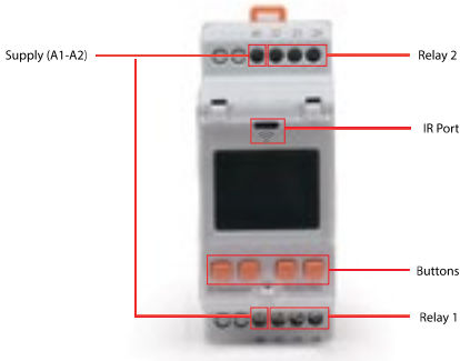
Figure 1-2 General view Meastro 121, 221, 321
